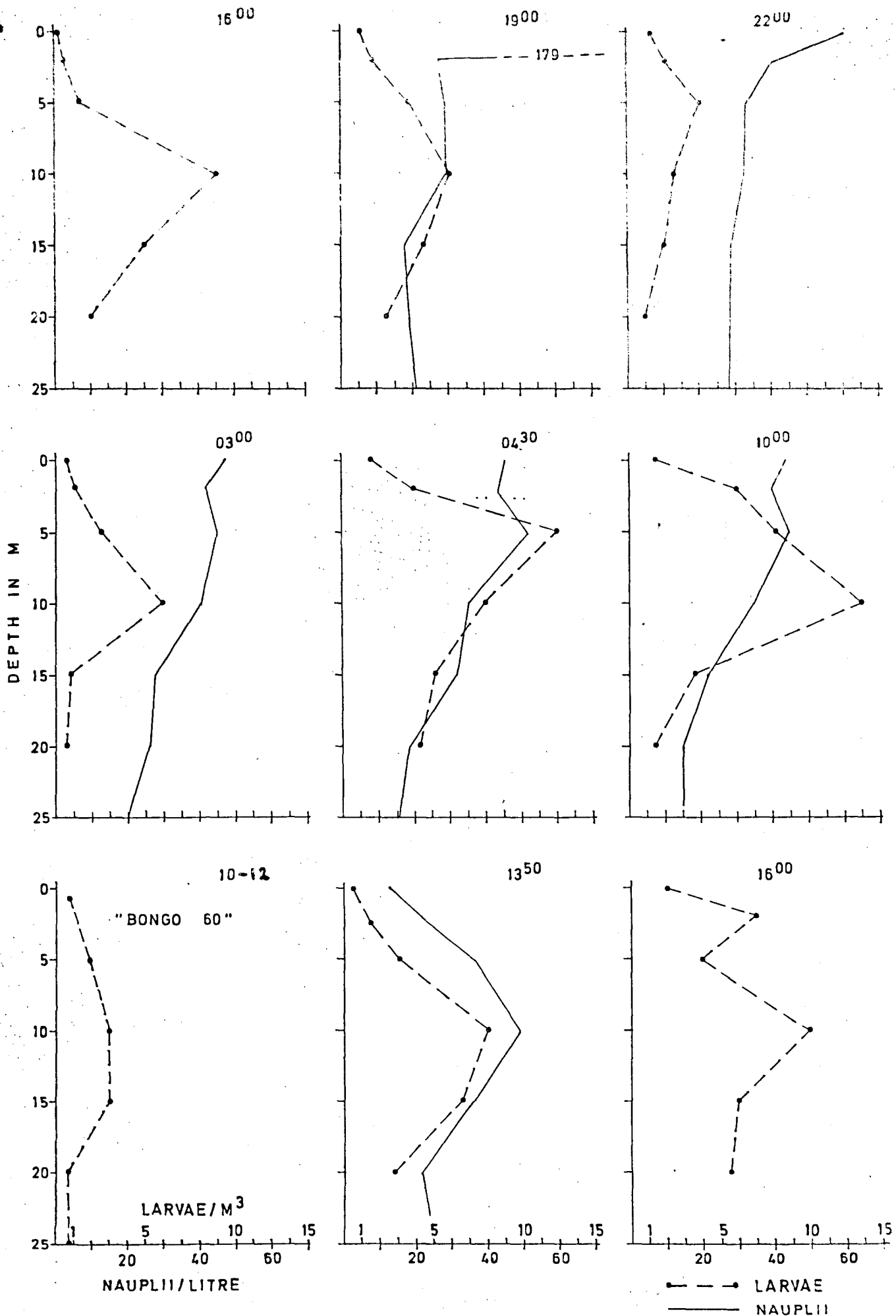
Fig. 13. Distribution of copepod nauplii and cod larvae in relation to depth, 18-19 May 1977 based upon commercial fish pump.
