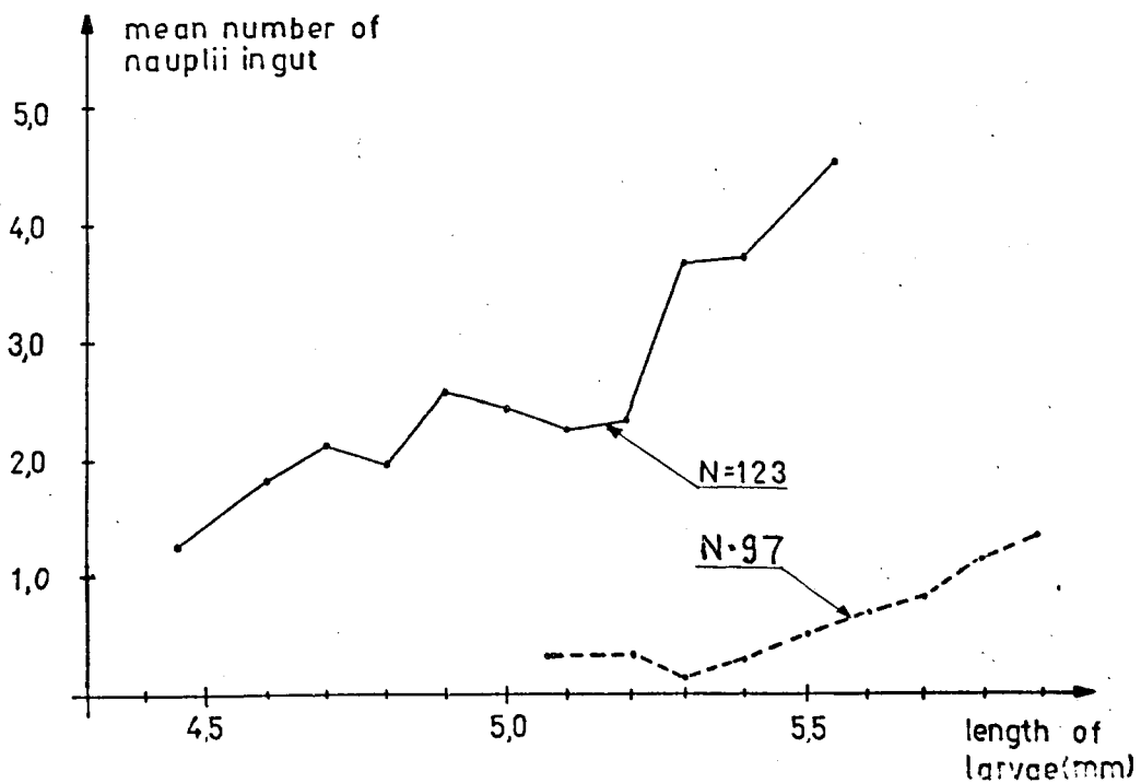
Fig.3. Mean number of nauplii in gut of cod larvae feeding on artemia salina in two experiment series carried out in 1975 (---) and 1976 (—)
