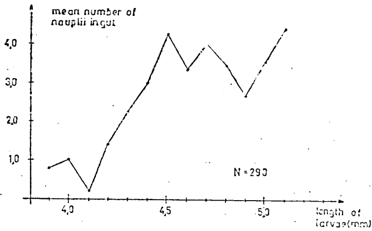
Fig. 4. Mean number of nauplii in the gut of cod larvae at different length of larvae observed in the basin experiment, on 30 March to 2 April 1976
