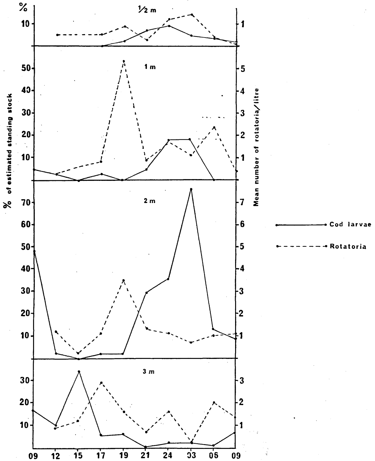
Fig. 11. Diurnal occurrence of cod larvae in four depths' presented as percentage of estimated standing stock (—) and of rotatorias as mean number per litre (----). From the basin experiment 3-4 May 1977.
