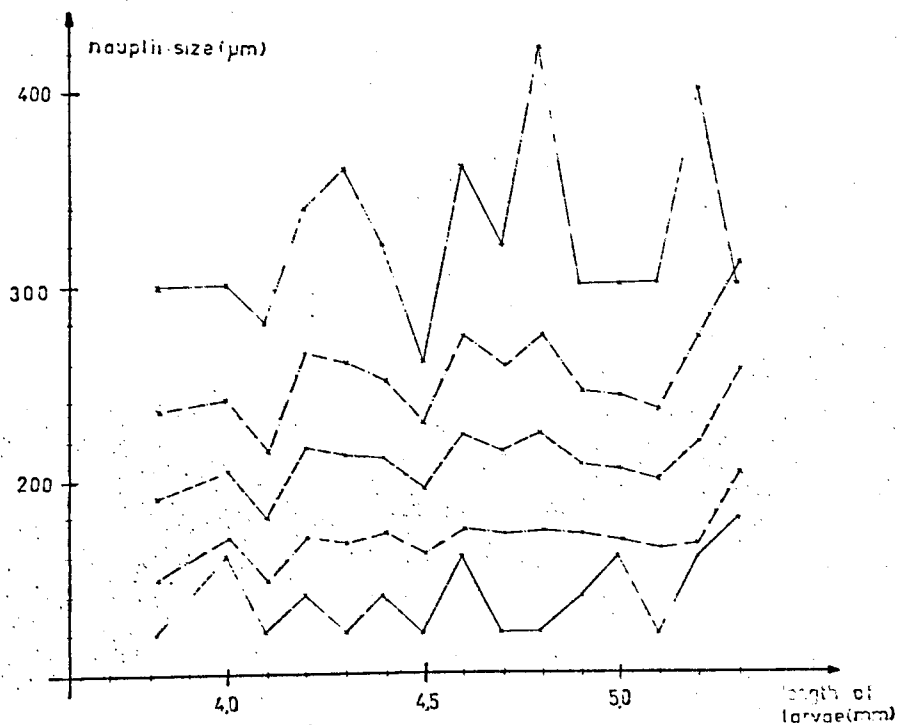
Fig. 8. Mean (-----), upper and lower standard deviation (-.-.-) and smallest and biggest (—) nauplii size observed in gut of larvae at different length. The larvae was caught at 15m depth 10-11 May 1977.
