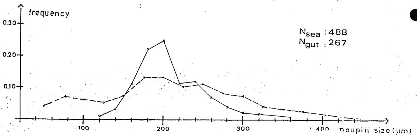
Fig. 10. Carapax-length distribution of copepod nauplii observed in the sea (---) and gut of larvae (—) at a 24 hour station in the Lofoten area 10-11 May 1977.
