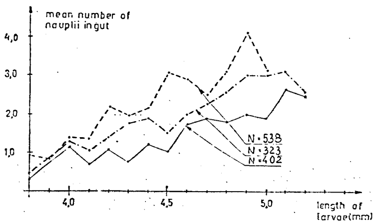
Fig. 6. The mean number of nauplii in gut of larvae at three 24 hour stations 3 May 1976 (—), 10-11 May 1977 (----) and 18-19 May 1977 (-.-.-)
