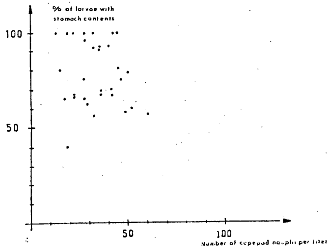
Fig. 18. Feeding incidence of larvae observed at the 24 hour station 18-19 May 1977.
